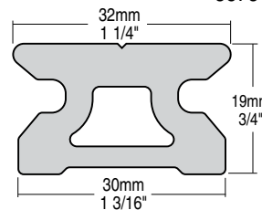
R32 Big Boat Traveller Schiene
